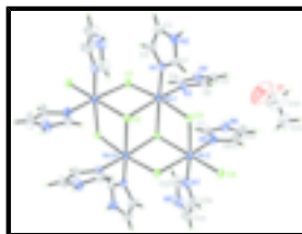
Fig. 1. The molecular structure of I with atom labels and 50% probability displacement ellipsoids for non-H atoms. [Symmetry code (A): -x, -y, -z + 1 ]
